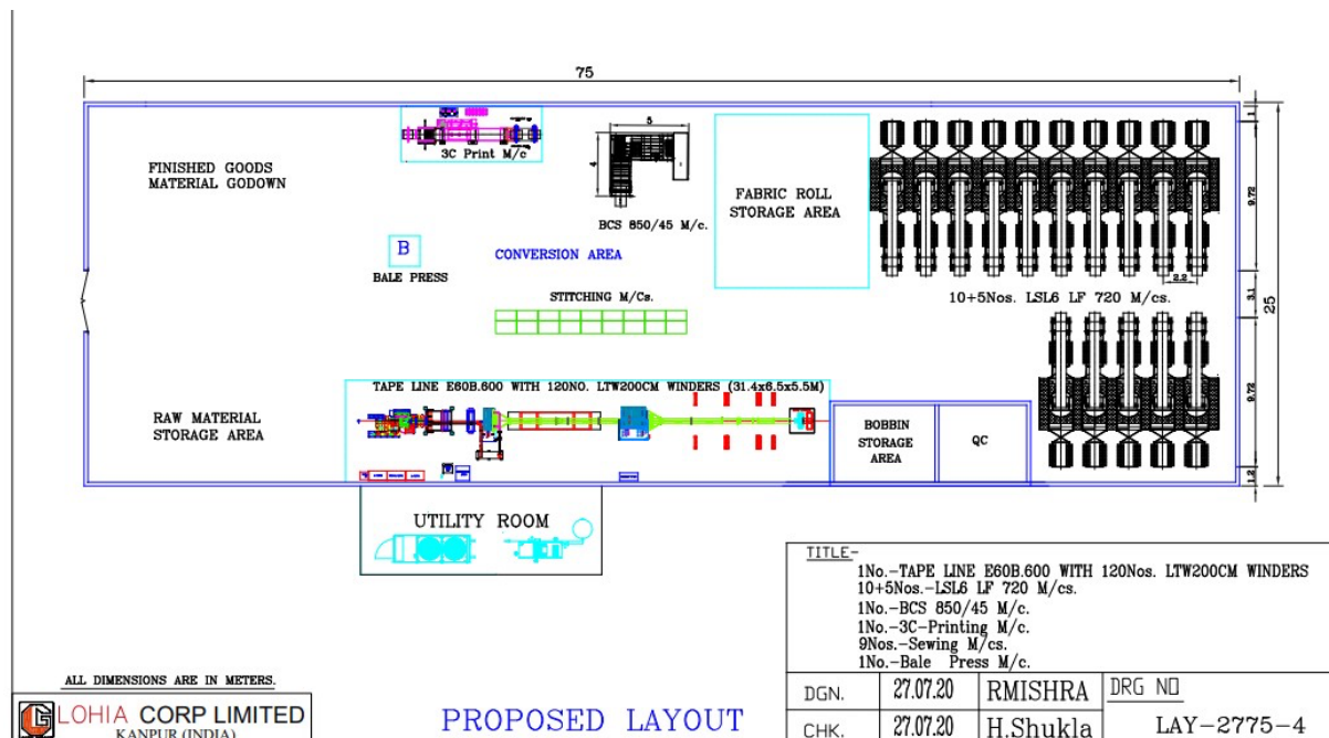
Figure 4: Proposed plant Layout
