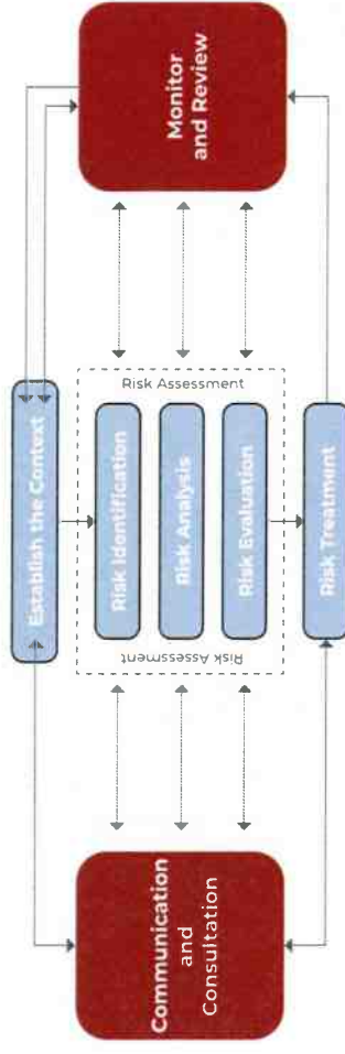
Figure 2: ERM Framework
