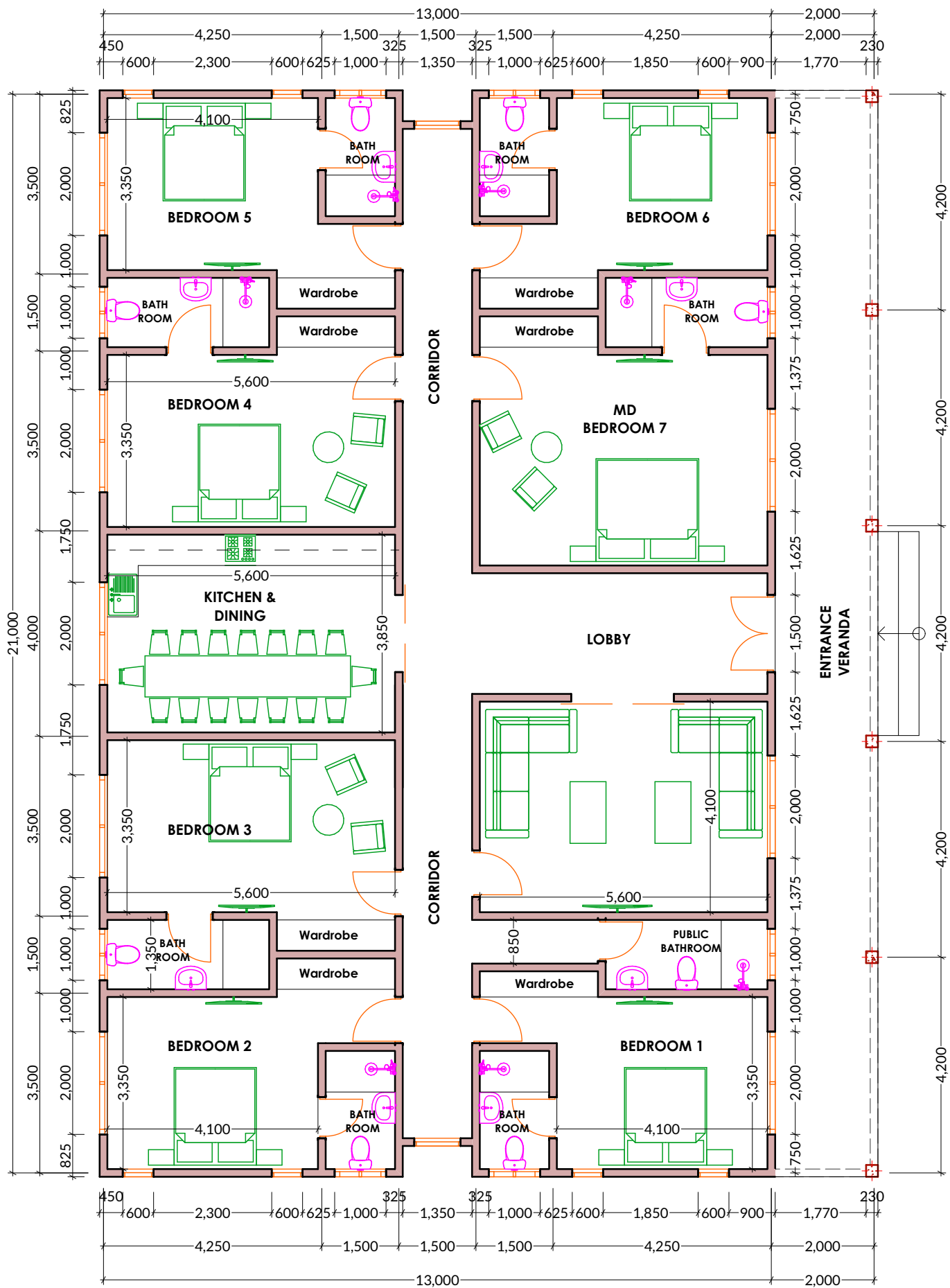
FLOOR PLAN (7 BEDROOMS)
