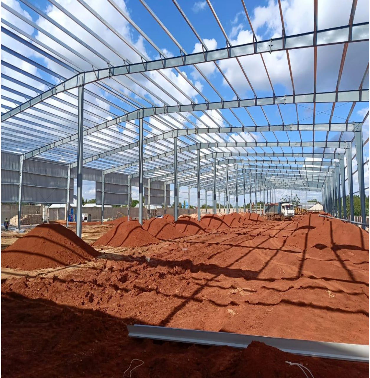
ERECTION OF COLUMNS AND BEAMS
